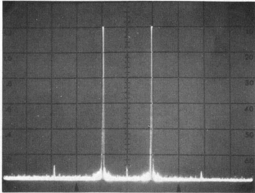
Fig. 3. Oscilloscope of spectrum analyzer presentation showing excellent carrier rejection in balanced modulator output of new mixer. A 50-Mc/s signal is being modulated by a 1-Mc/s signal. Vertical scale is 10 dB/cm so carrier rejection is well above 50 dB. Horizontal scale is 1 Mc/s/cm.
