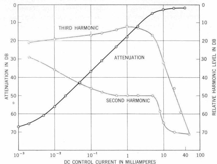
Fig. 8. Typical attenuation (solid line) at mixer output ("R" port) of a signal applied to "L" port as a function of a dc control current applied to "X" port. (See also Fig. 4.) 0 \text{ dB} is +3 \text{ dBm} input level. Input signal is 50 \text{ Mc/s} . Shaded lines show relative harmonic content in mixer output vs. control current for a typical mixer. 1 \text{ Mc/s} input signal level at +3 \text{ dBm} .
