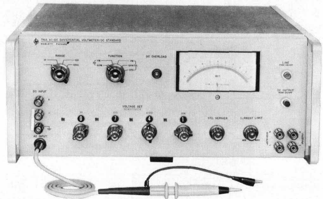
Fig. 4. New -hp- Model 741A AC/DC Differential Voltmeter/DC Standard has low capacitance probe for ac input. Probe and dc input and output are floating. Four VOLTAGE SET controls set resistive divider and push-buttons concentric with VOLTAGE SET knobs select sensitivity of front panel meter. RANGE switch sets illuminated decimal point indicators. OVERLOAD indicator lights if input voltage exceeds selected range or if output current exceeds selected limit. Overload protection to 1000 volts is provided on all ranges.
