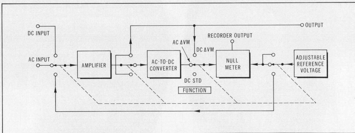
Fig. 2. Basic elements of AC-DC Differential Voltmeter/DC Standard. Function switch is set for ac differential voltmeter mode (AC \Delta VM), in which Null Meter indicates difference (differential) between Adjustable Reference Voltage and dc
